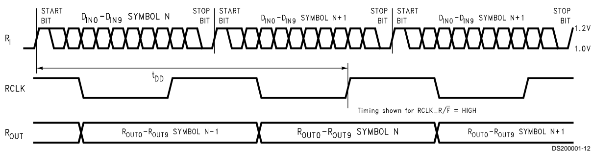
FIGURE 12. Deserializer Delay
