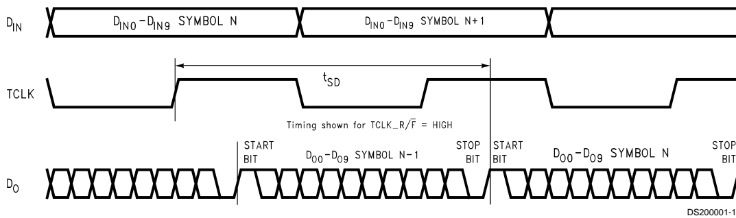
FIGURE 11. Serializer Delay
