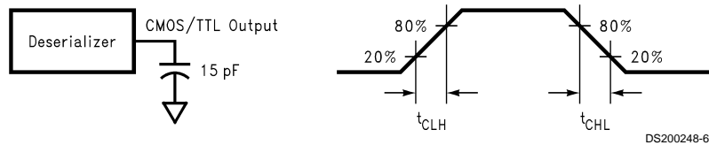
FIGURE 5. Deserializer CMOS/TTL Output Load and Transition Times
