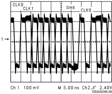
DIN8 Held Low-DIN9 Held High Creates an RMT Pattern FIGURE 1. RMT Patterns Seen on the Bus LVDS Serial Output
