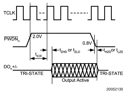
FIGURE 7. Individual Channel Power up Time, t_{ICR}
