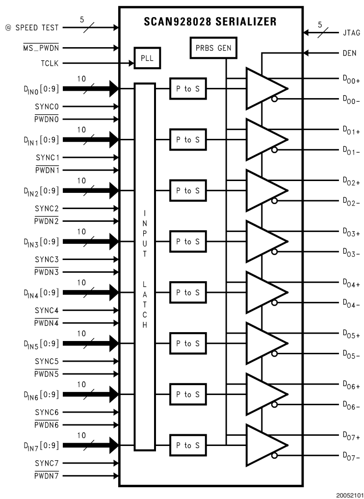
FIGURE 11. SCAN928028 Functional Block Diagram
