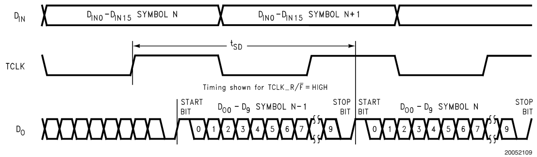
FIGURE 8. Serializer Delay
