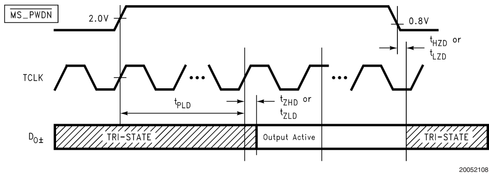
FIGURE 6. Serializer PLL lock Time and \overline{\text{MS\_PWDN}} TRI-STATE Delays
