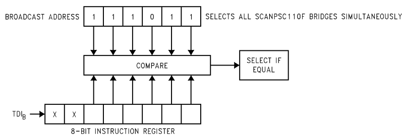
FIGURE 7. Broadcast Addressing: Address Loaded into Instruction Register
