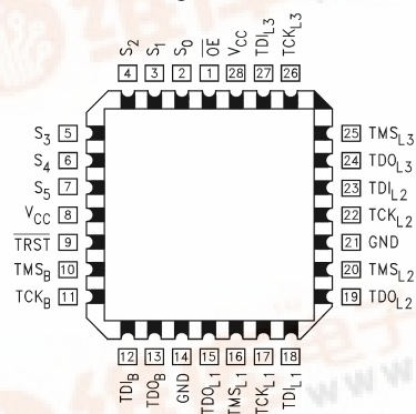
Pin Assignment for LCC
