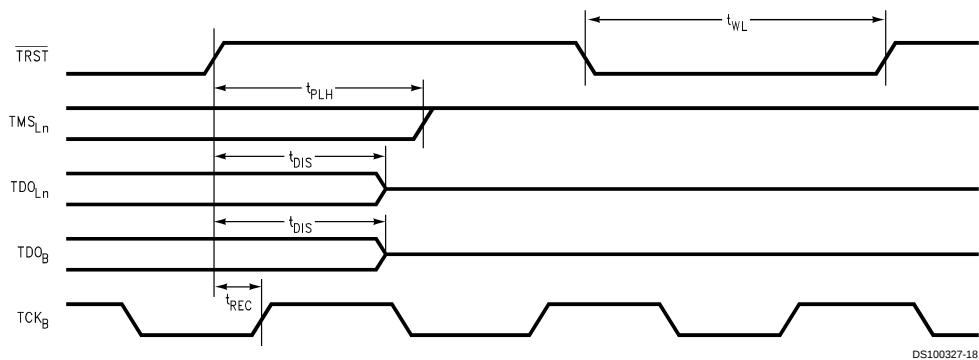
FIGURE 15. Reset Waveforms
