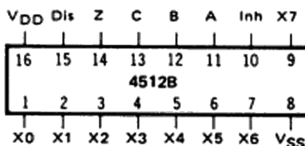
CONNECTION DIAGRAM (all packages)
