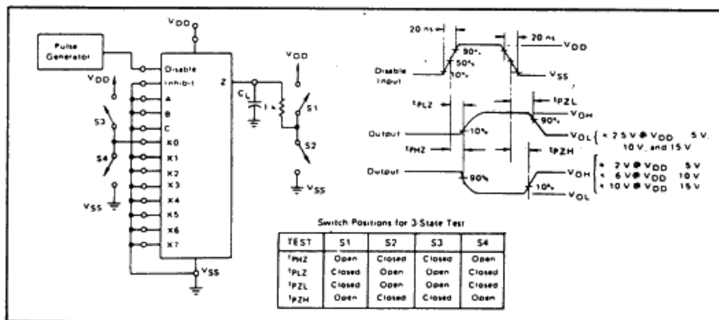
3-State AC Test Circuit and Waveform
