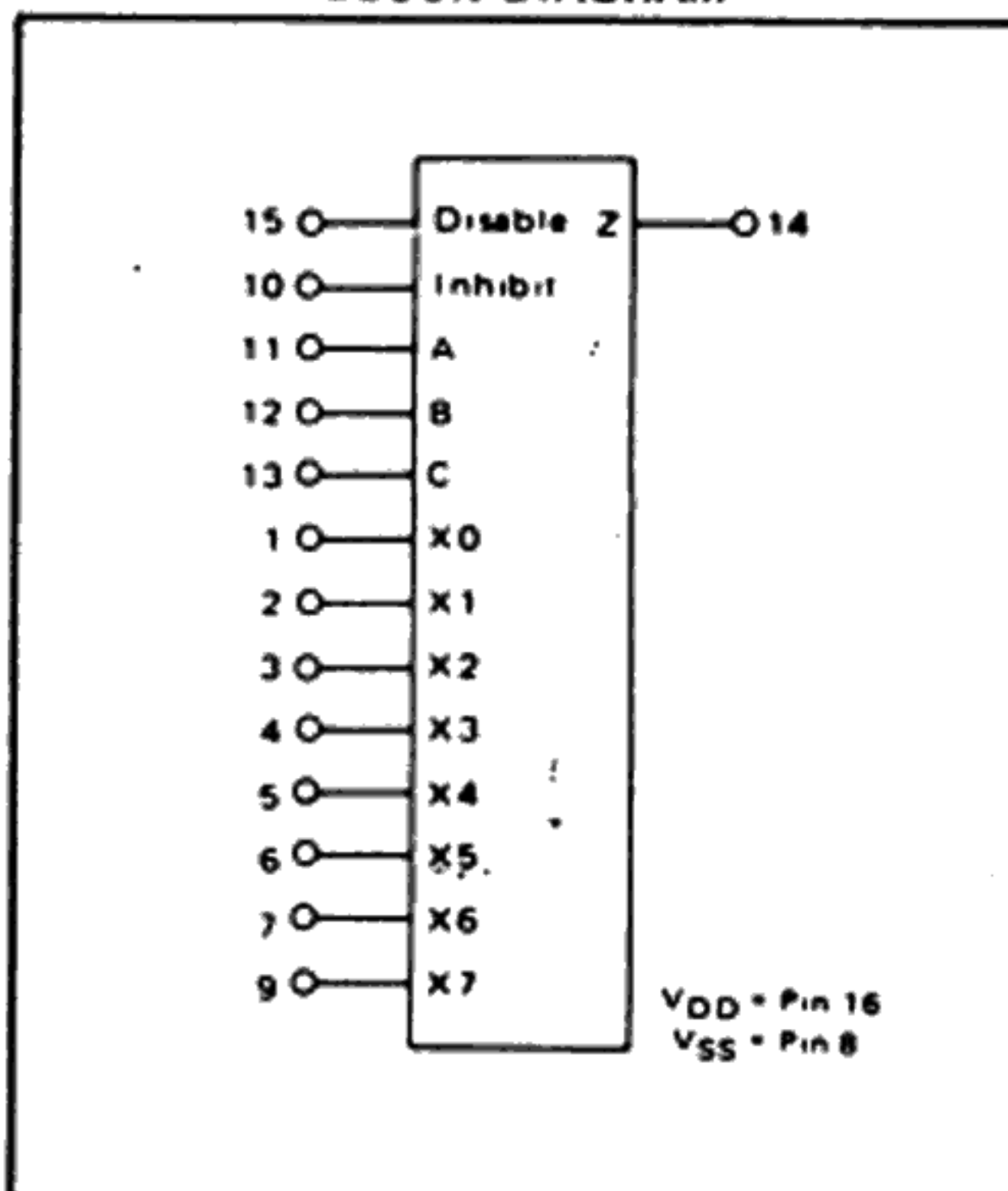
BLOCK DIAGRAM
