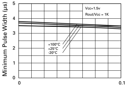
Lowest Voltage Level of Trigger Pulse ( \times V_{CC} ) Minimum Pulse Width Required for Triggering
