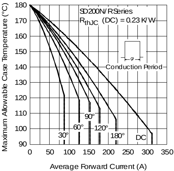
Fig. 2 - Current Ratings Characteristics
