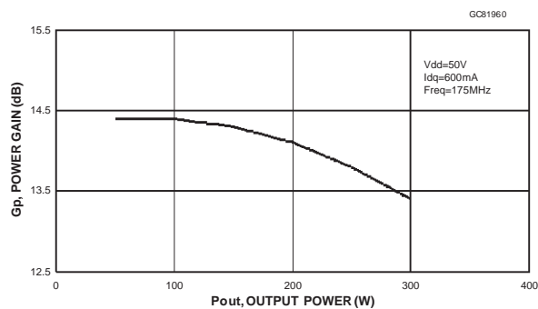
1 dB Compression
