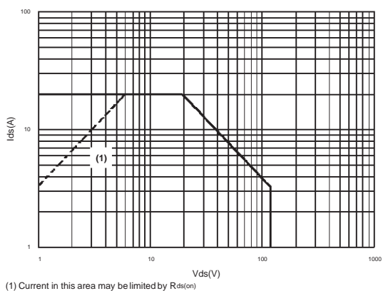
DC Safe Operating Area
