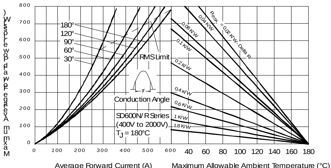
Fig. 4 - Current Ratings Characteristics
