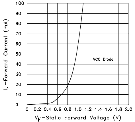
I_F vs V_F Characteristic
