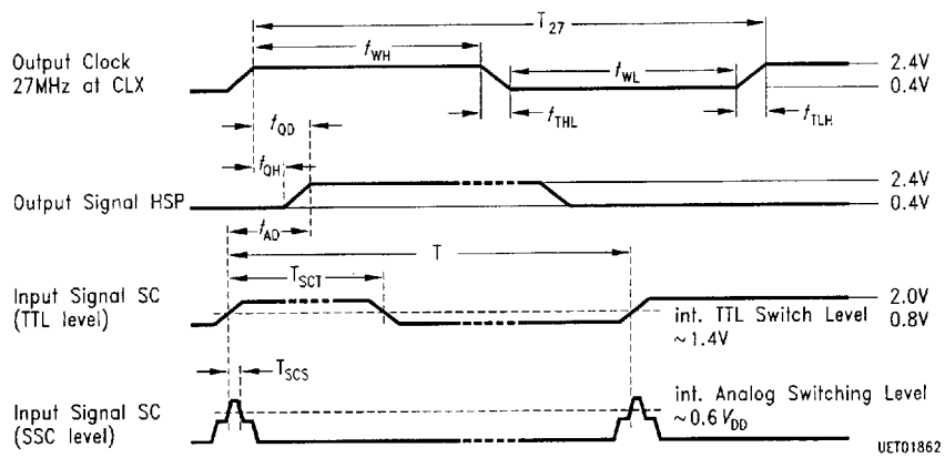
Timing Diagram 1 Timing of SDA 9086-3
