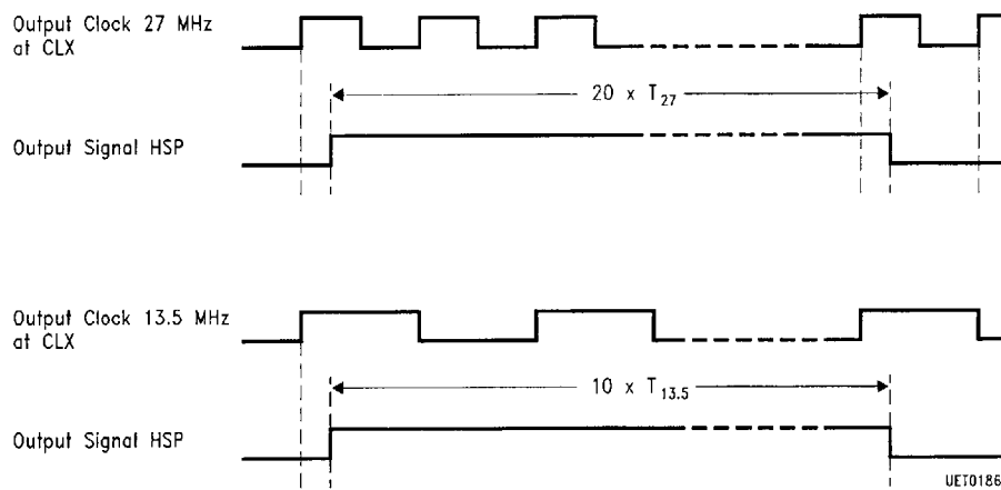
Timing Diagram 2 HSP Pulse Width
