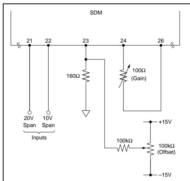
FIGURE 11. Unipolar Calibration.
