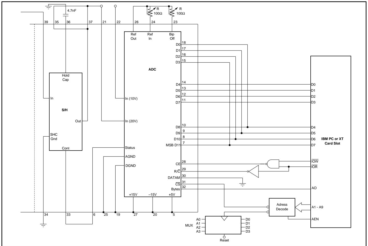
FIGURE 19c. IBM PC SDM Interface.
