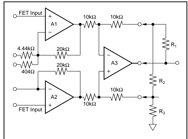
FIGURE 5. Increasing Output Amplifier Gain.
