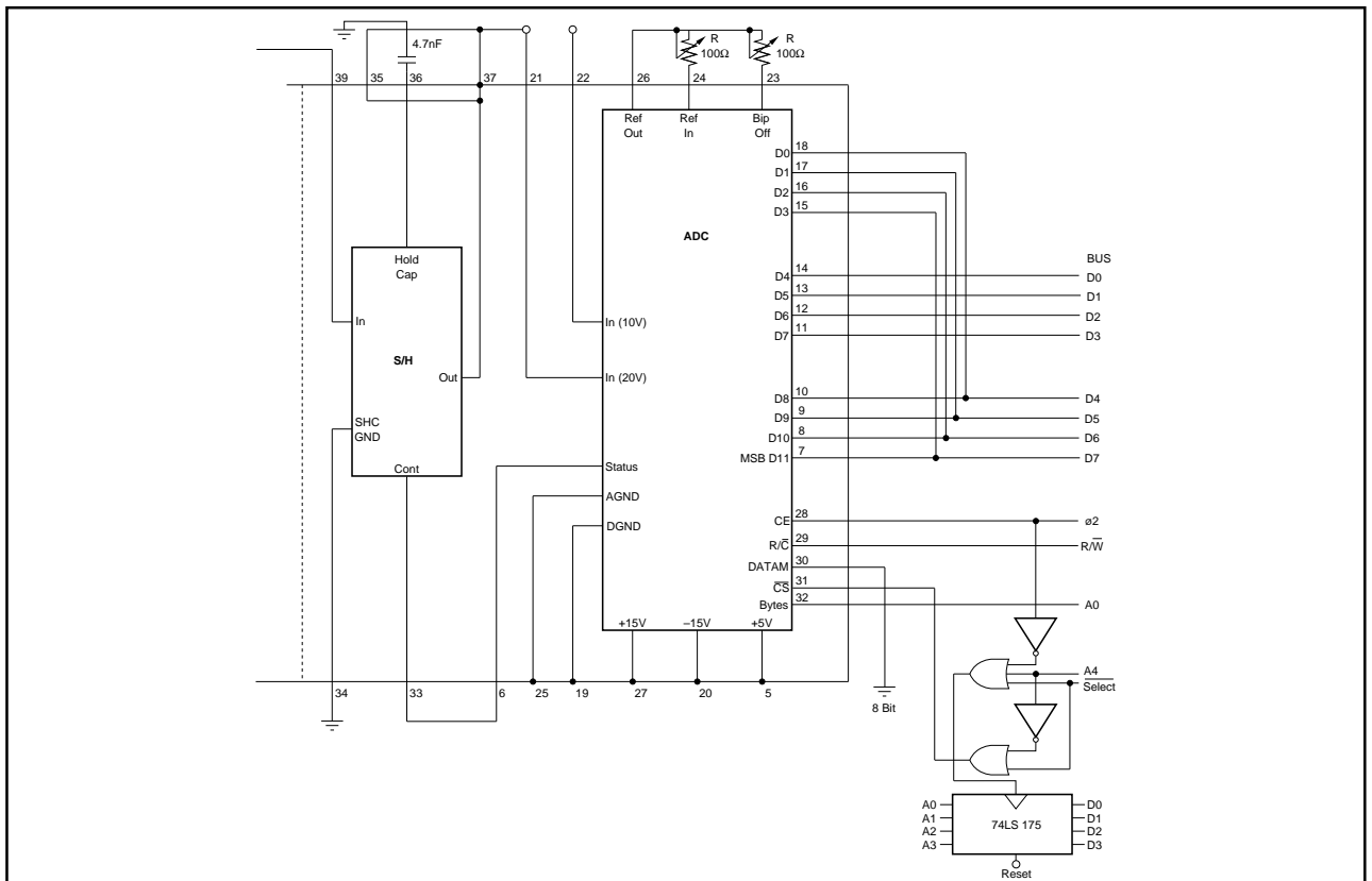
FIGURE 20. SDM on the 6502 BUS.
