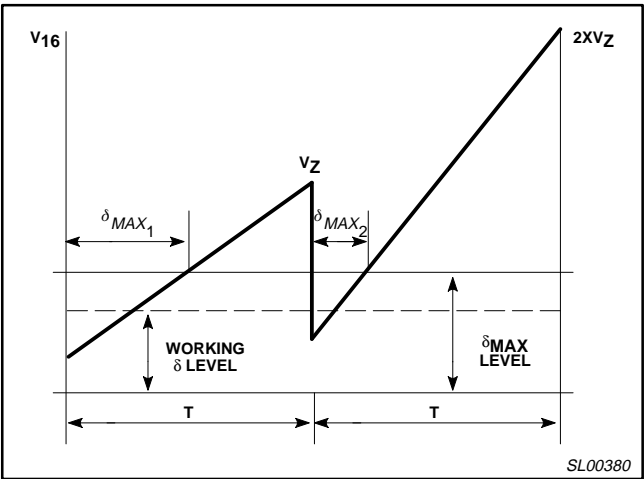
Figure 21. Feed-Forward Circuitry
