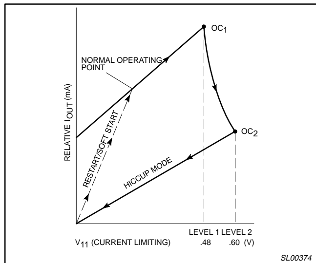
Figure 15. Output Characteristics
