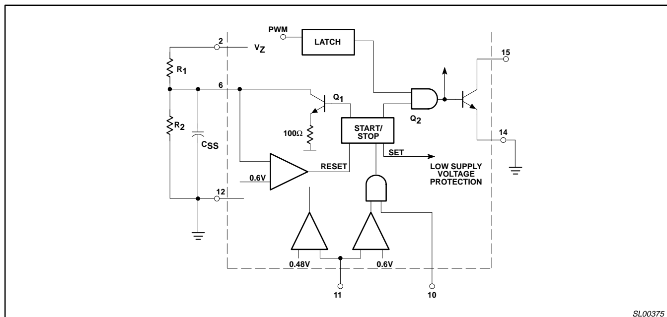
Figure 16. Start-Stop Circuit
