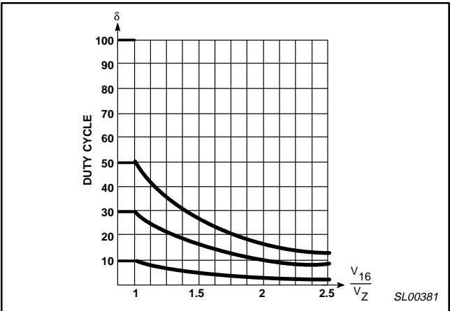
Figure 22. Feed-Forward Regulation
