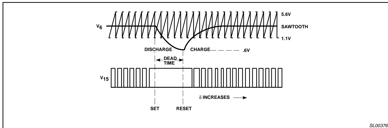
Figure 17. Start-Stop Circuit
