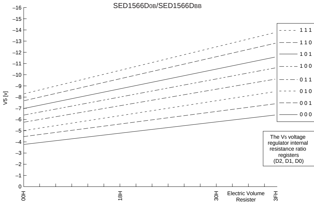
Figure 12: SED1566D0B/SED1566D0B (1) For Models Where the Thermal Gradient = -0.05%/°C
