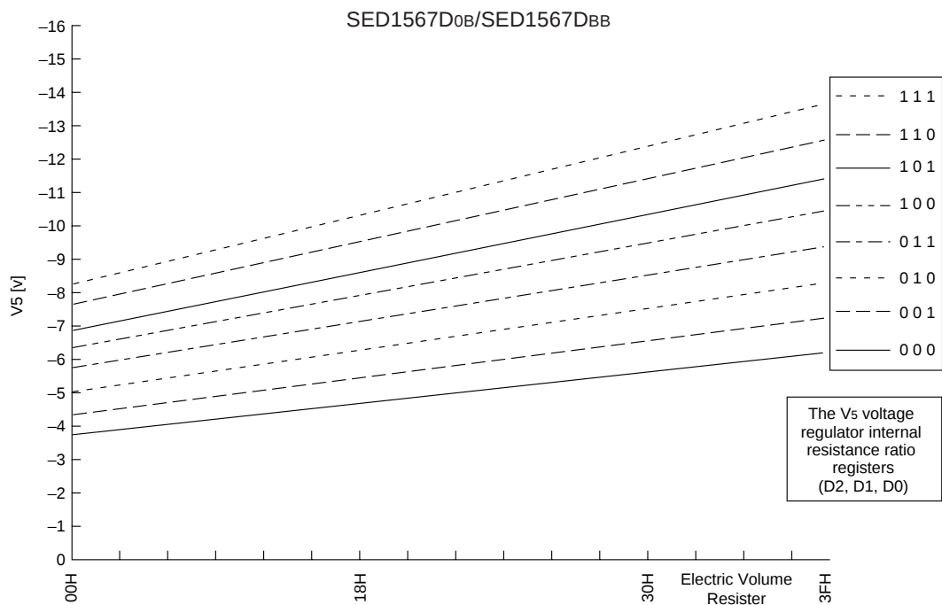
Figure 15: SED1567D0B/SED1567DBB (1) For Models Where the Thermal Gradient = -0.05\%/^{\circ}\text{C}
