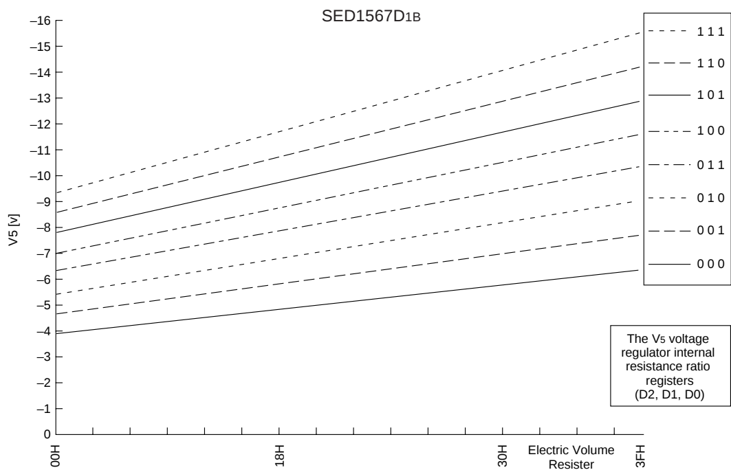
Figure 16: SED1567D1B (2) For Models Where the Thermal Gradient = -0.2\%/^{\circ}\text{C}
