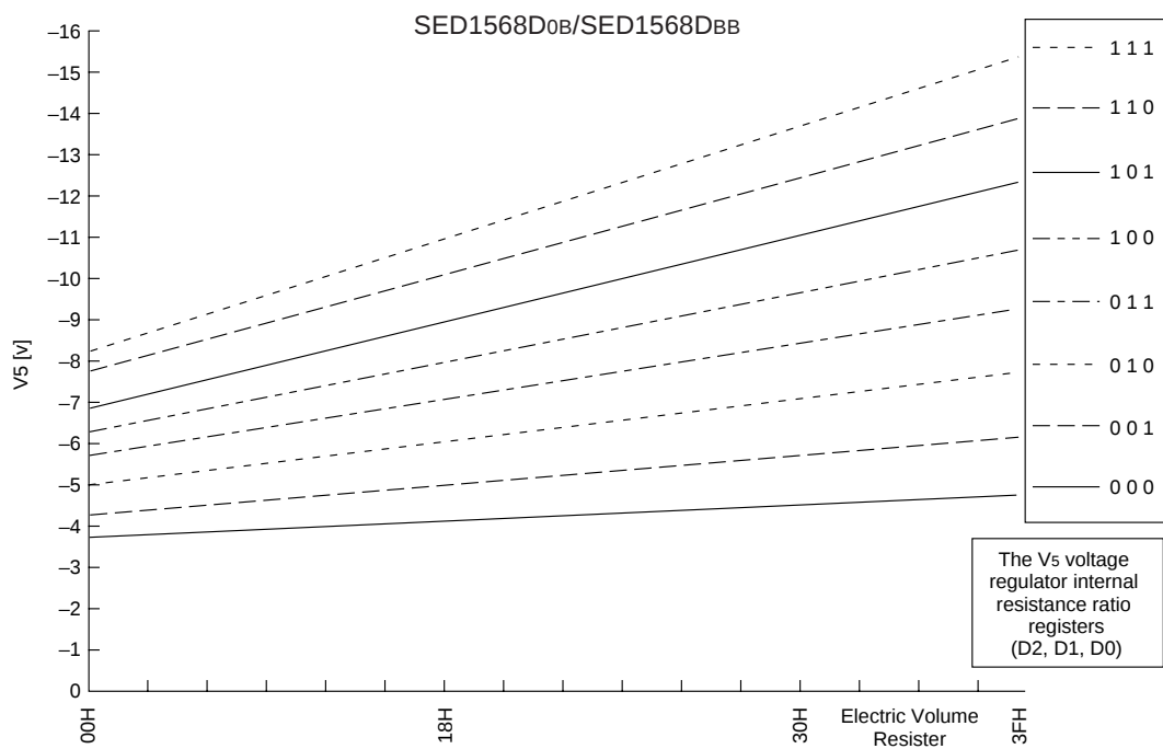
Figure 18: SED1568D0B/SED1568DBB (1) For Models Where the Thermal Gradient = -0.05%/°C
