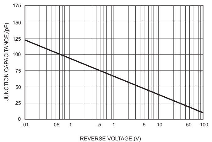
FIG.6-TYPICAL JUNCTION CAPACITANCE
