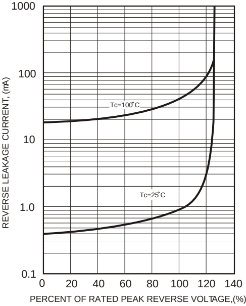
FIG.4-TYPICAL REVERSE CHARACTERISTICS
