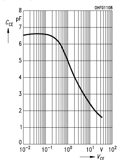
Collector-emitter capacitance
