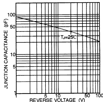
FIG. 4-TYPICAL JUNCTION CAPACITANCE
