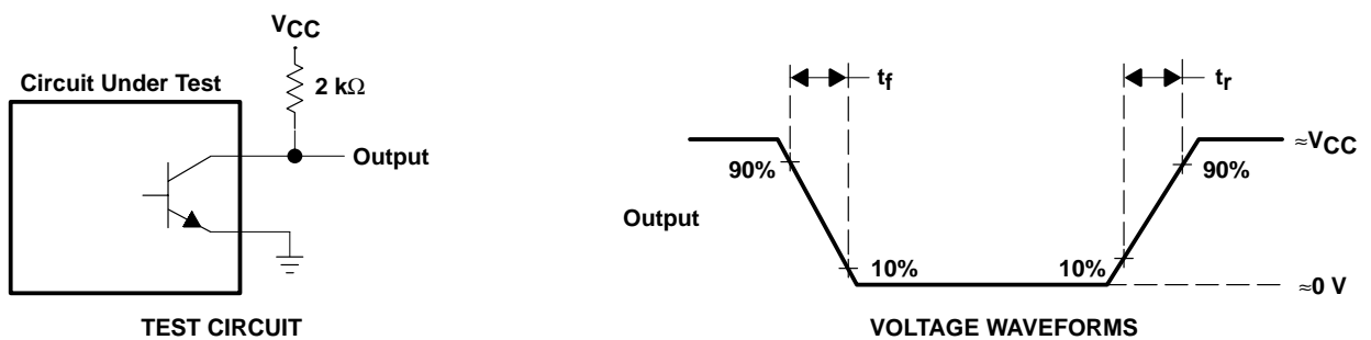
Figure 2. Switching Times
