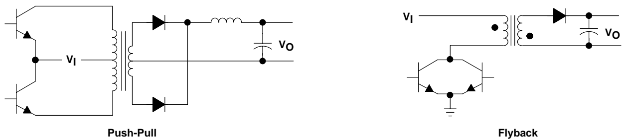
Figure 11. Transformer-Coupled Outputs
