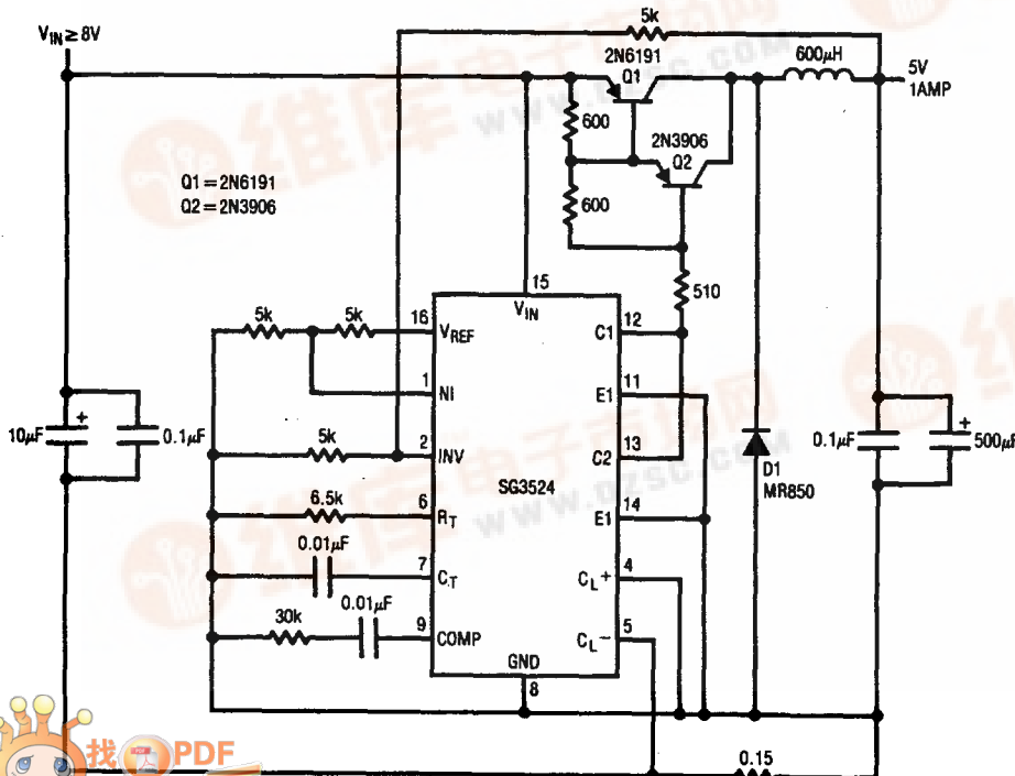
5V, 1 Amp Regulator
