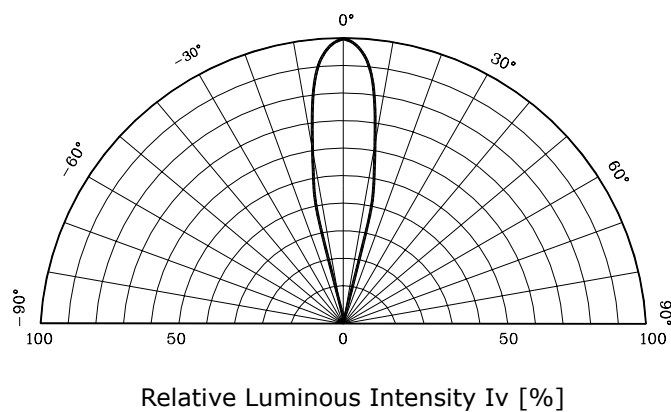
Fig. 5 Radiation Diagram
