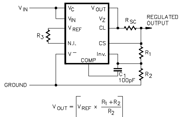
FIGURE 8 - BASIC HIGH VOLTAGE REGULATOR V_{OUT} = 7V \text{ TO } 37V
