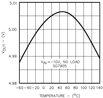
FIGURE 3. TEMPERATURE COEFFICIENT
