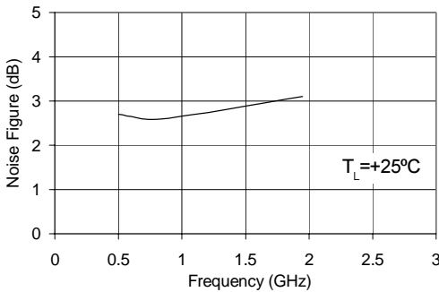
Noise Figure vs. Frequency V D = 2.6 V, I D = 20 mA
