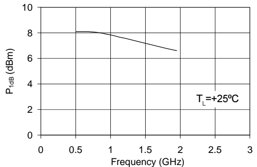
P 1dB vs. Frequency V D = 2.6 V, I D = 20 mA
