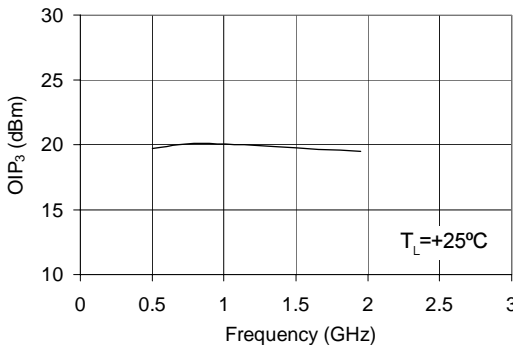
OIP 3 vs. Frequency V D = 2.6 V, I D = 20 mA
