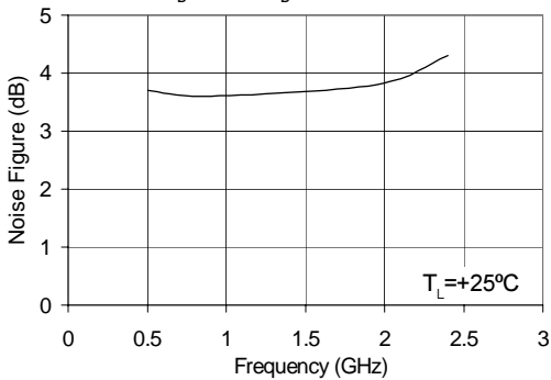
Noise Figure vs. Frequency V D = 2.6 V, I D = 35 mA (Typ.)
