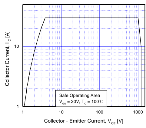
Fig 16. Turn-Off SOA
