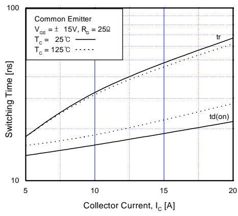
Fig 11. Turn-On Characteristics vs. Collector Current
