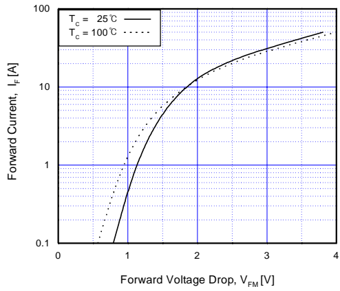
Fig 18. Forward Characteristics
