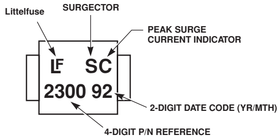
SGT2300SC (TOP VIEW - NOT TO SCALE)
