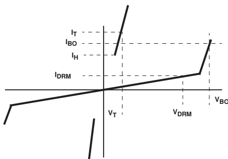
FIGURE 1. V-I CHARACTERISTICS
