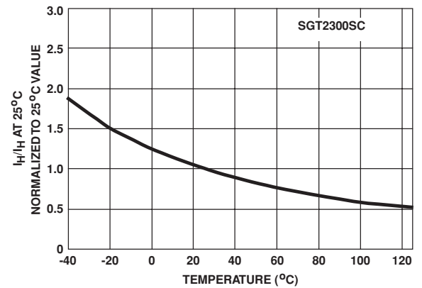
FIGURE 8. TYPICAL HOLDING CURRENT vs JUNCTION TEMPERATURE
