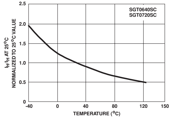
FIGURE 6. TYPICAL HOLDING CURRENT vs JUNCTION TEMPERATURE
