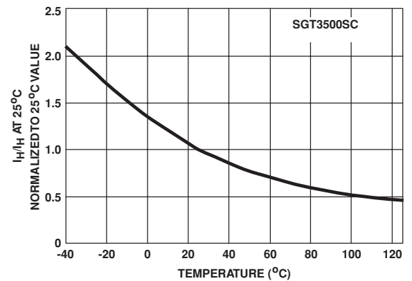
FIGURE 10. TYPICAL HOLDING CURRENT vs JUNCTION TEMPERATURE
