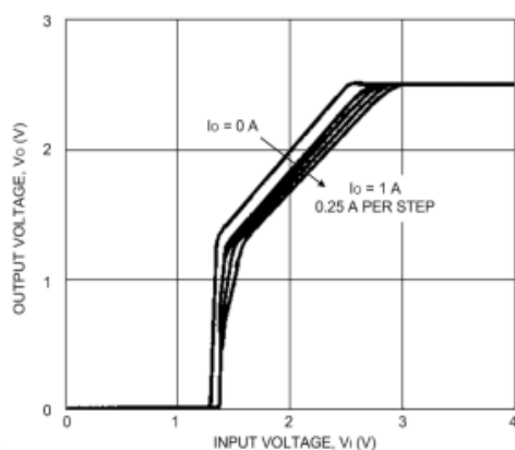
Low-Voltage Behavior
