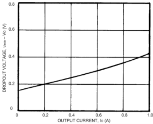
Dropout Voltage
