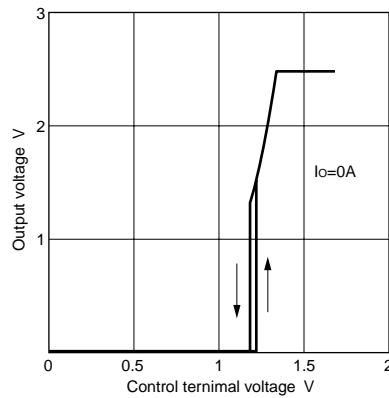
Control terminal voltage vs. Output voltage
