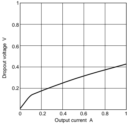
Dropout voltage
