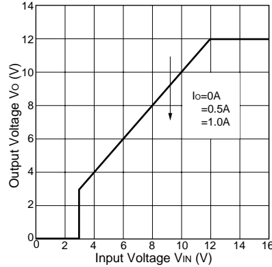
Rise Characteristics(SI-3120F)
