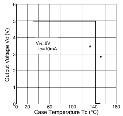
Thermal Protection Characteristics(SI-3050F)
