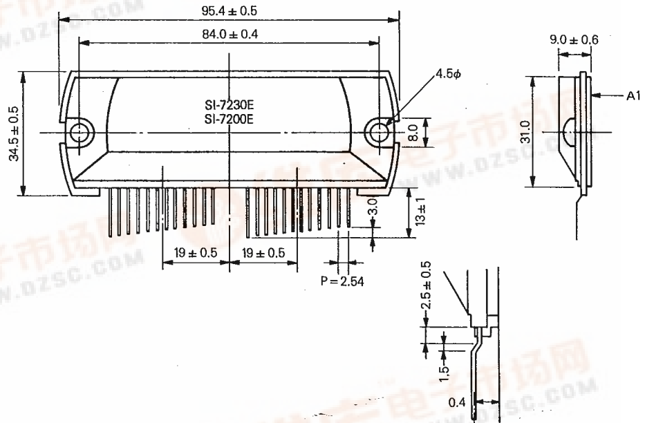
Outline Drawings Unit: mm
