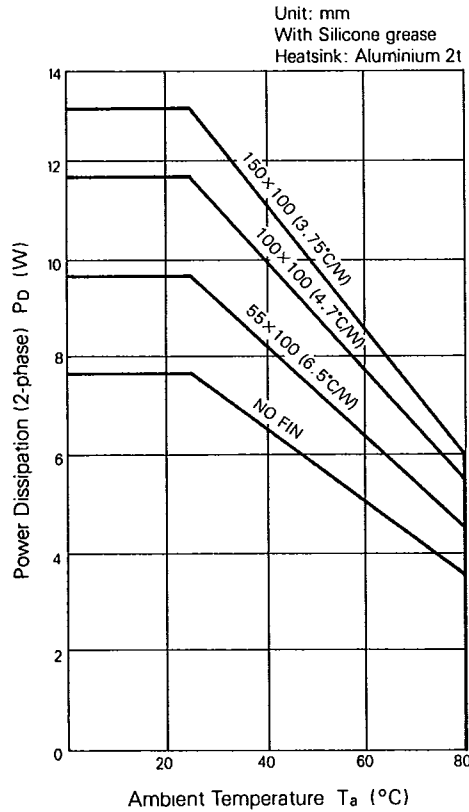
SI-7200E Derating
