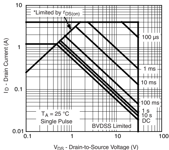
V_{DS} - Drain-to-Source Voltage (V) * V_{GS} > minimum V_{GS} at which r_{DS(on)} is specified Safe Operating Area, Junction-to-Ambient
