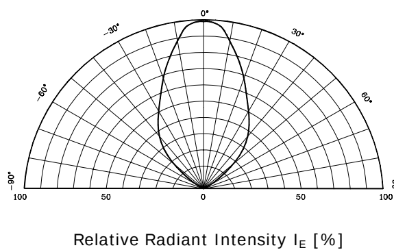
Fig. 5 Radiation Diagram
