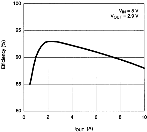
FIGURE 9. Efficiency
