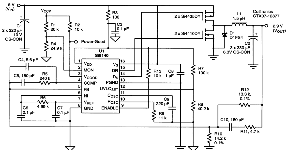
FIGURE 1. 2.9 V @ 10 A
