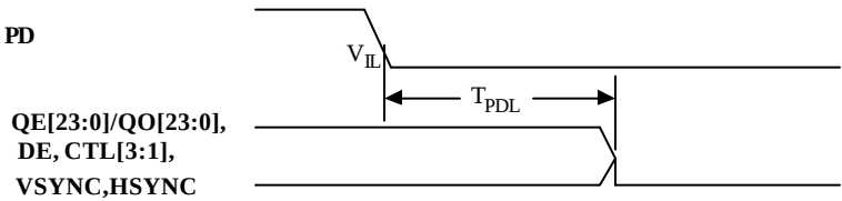
Figure 5. Output Signals Disabled Timing from PD Active
