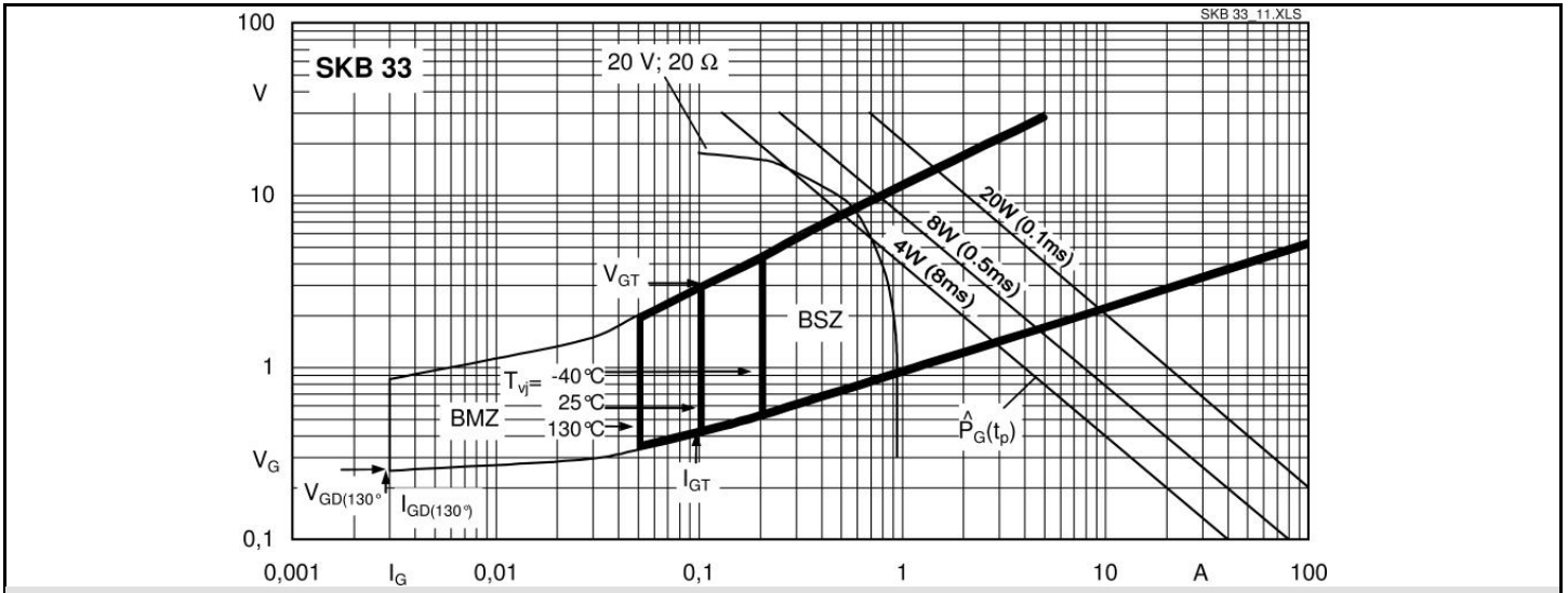
Fig. 11 Gate characteristics of a thyristor device
