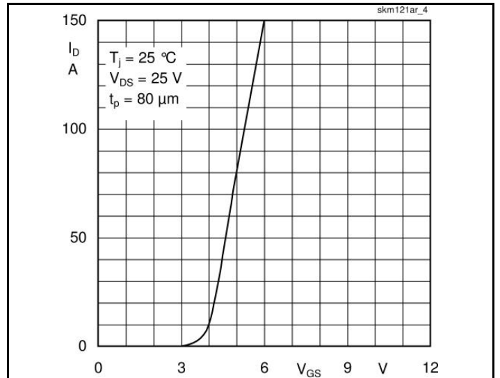
Fig. 4 Transfer characteristic
