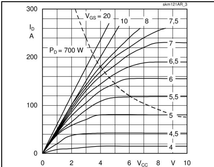
Fig. 3 Output characteristic
