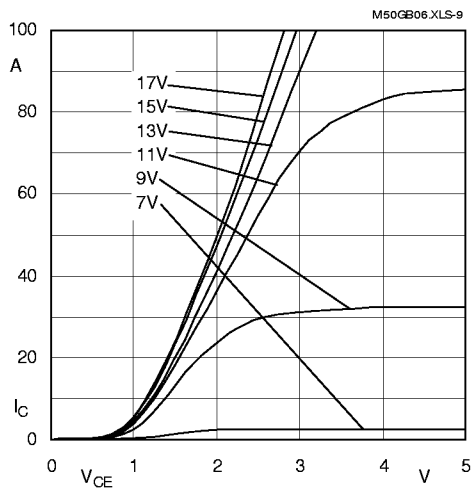
Fig. 9 Typ. output characteristic, t_p = 250 μs; T_j = 25 °C
