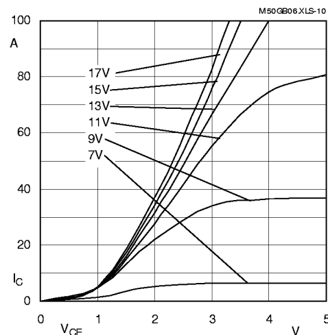
Fig. 10 Typ. output characteristic, t_p = 250 μs; T_j = 125 °C
