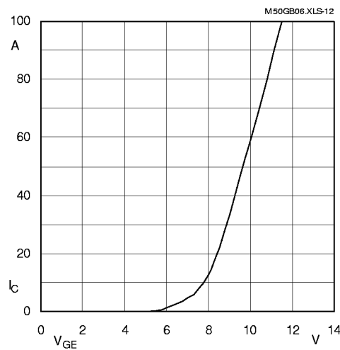
Fig. 12 Typ. transfer characteristic, t_p = 80 μs; V_{CE} = 20 V
