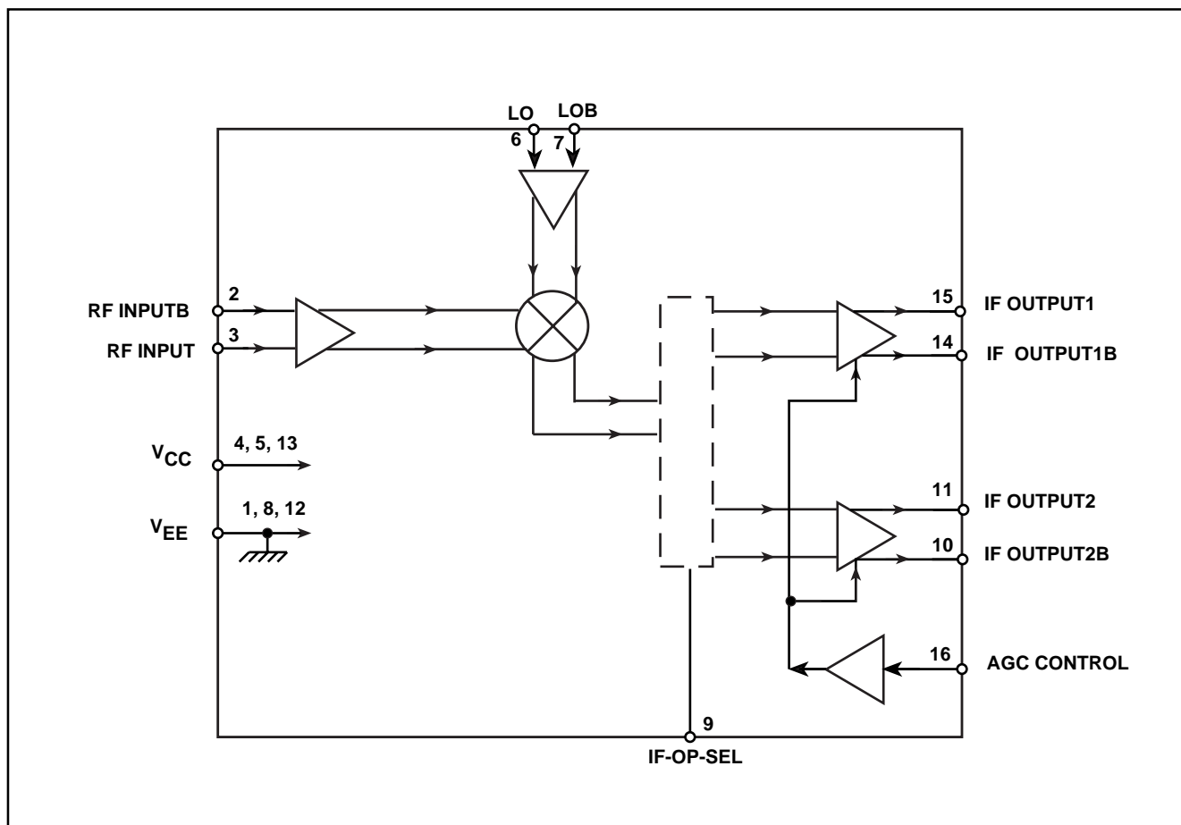
Fig. 2 Block diagram
