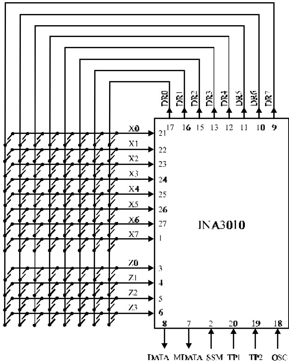
Figure 1. Keyboard interconnection
