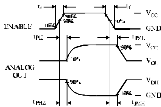
Figure 2. Switching Waveforms
