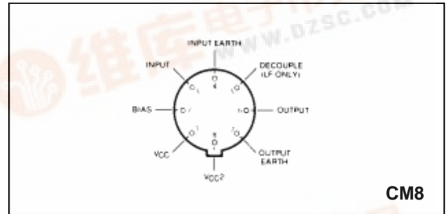
Fig.1 Pin connections
