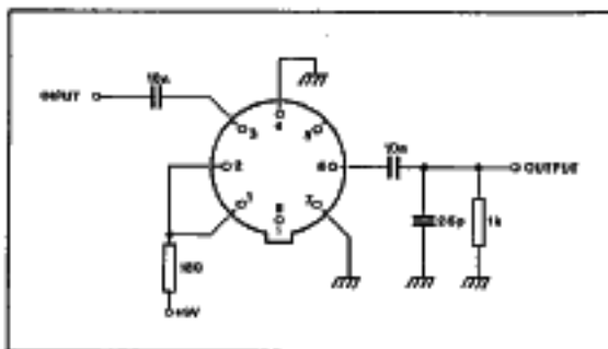
Fig. 4 Test circuit
