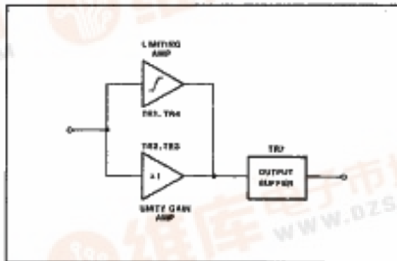
Fig. 3 Block diagram
