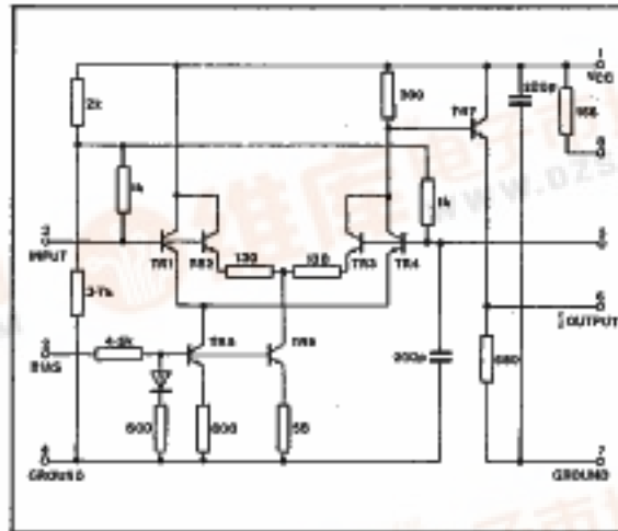
Fig. 2 Circuit diagram
