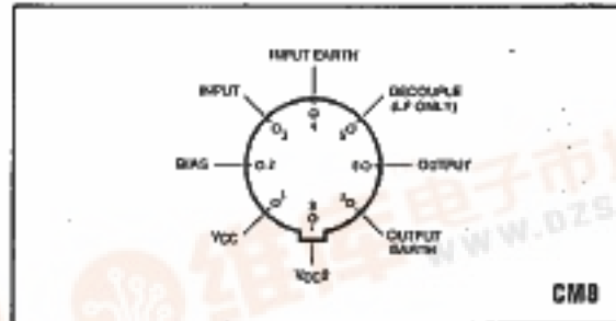
Fig. 1 Pin connections
