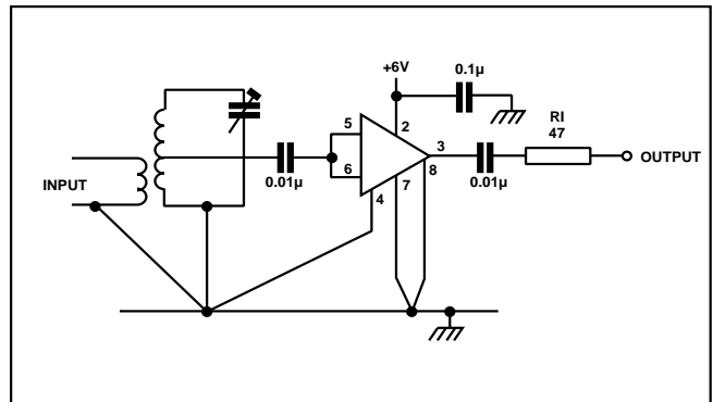
Fig.7 RF preamplifier
