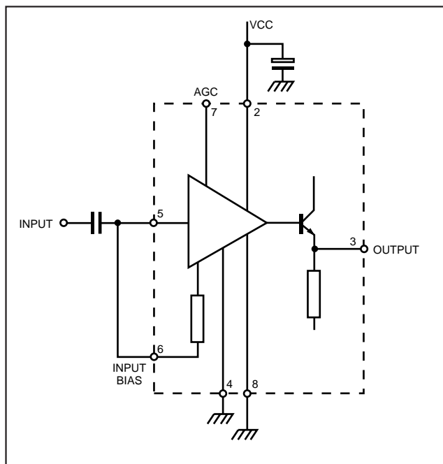
Fig.2 Block diagram
