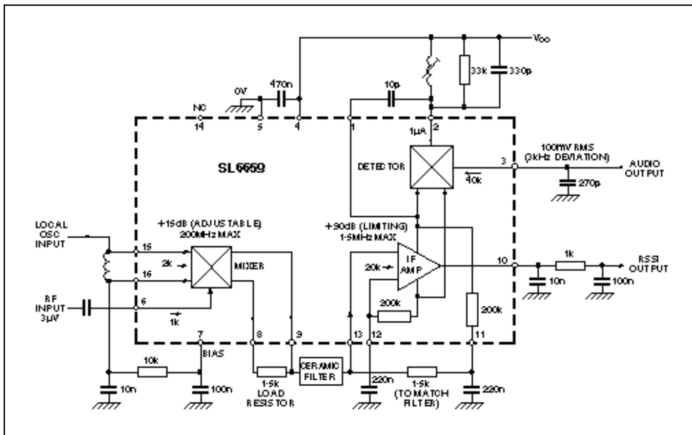
Fig. 2 Block diagram
