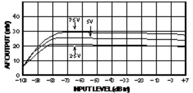
Fig. 7 Audio output v. input and supply voltage at +25°C
