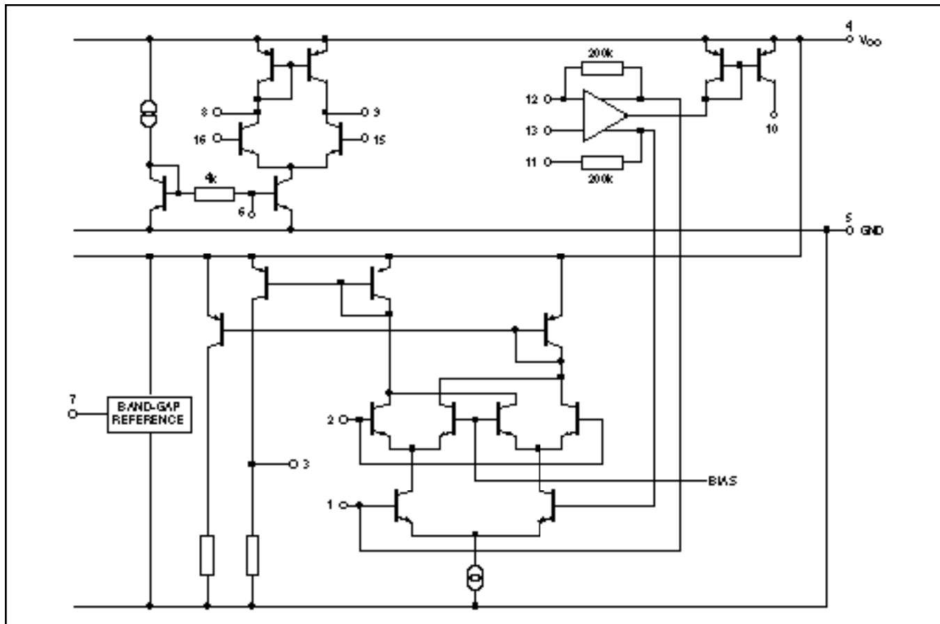
Fig. 3 Internal schematic
