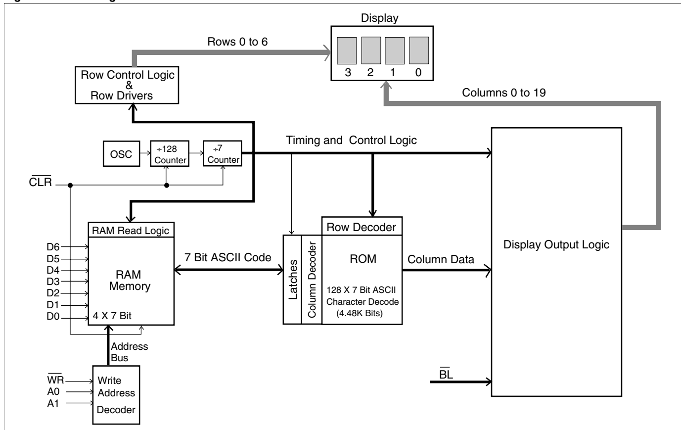
Figure 6. Block Diagram
